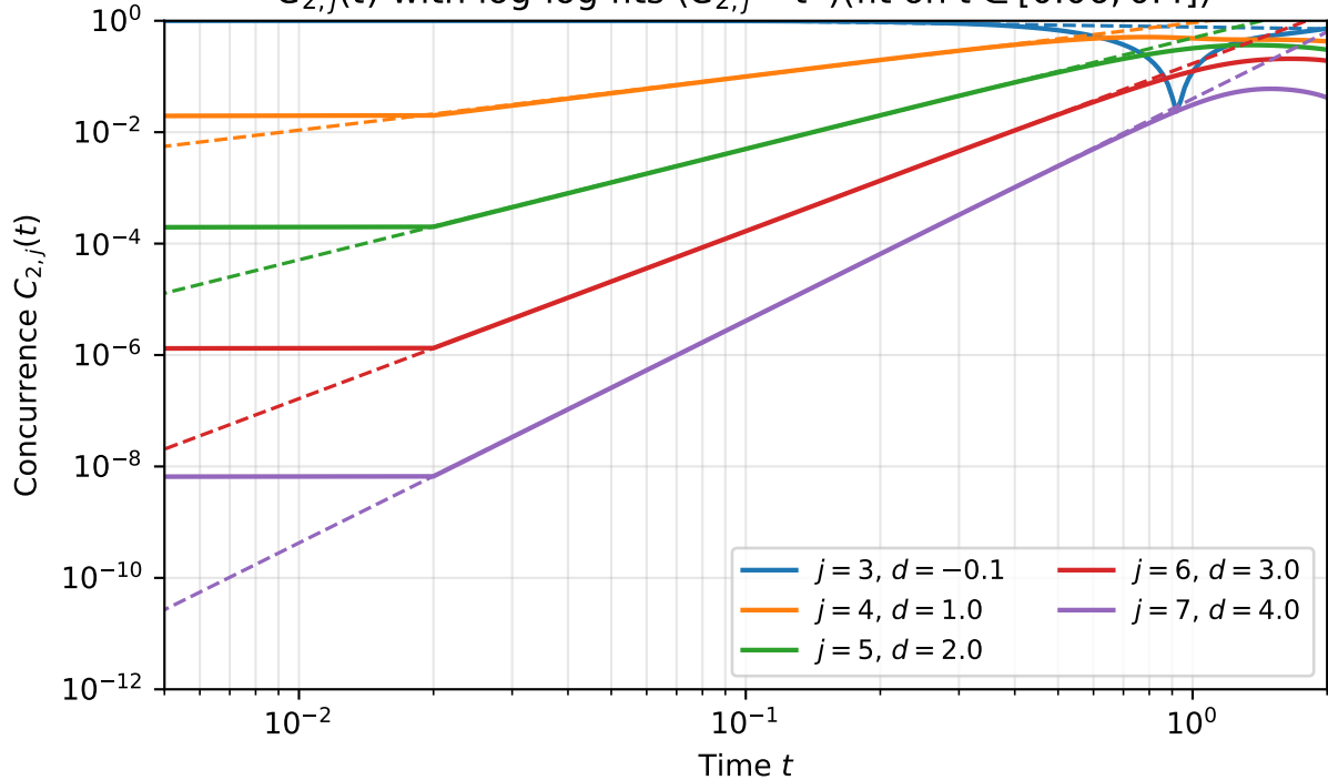
C_{2,j}(t) with log-log fits ( C_{2,j} \sim t^d )(fit on t \in [0.06, 0.4] )
